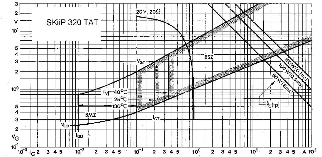
Fig. 10a Gate trigger characteristics (per thyristor)
