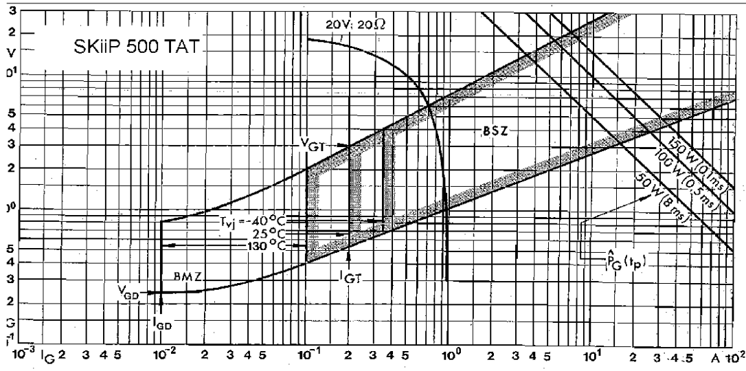
Fig. 10c Gate trigger characteristics (per thyristor)
