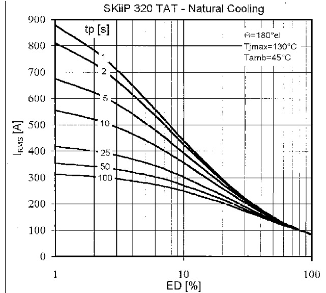
Fig. 2a Maximum rms current vs. duty cycle
